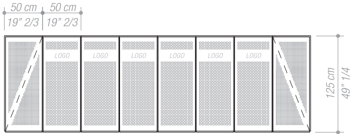
4 meters ramp
