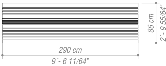
Backrest + Seat
