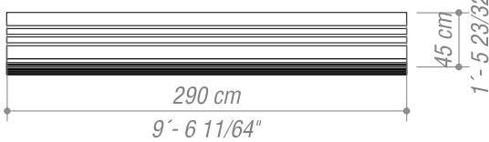
Backrest
